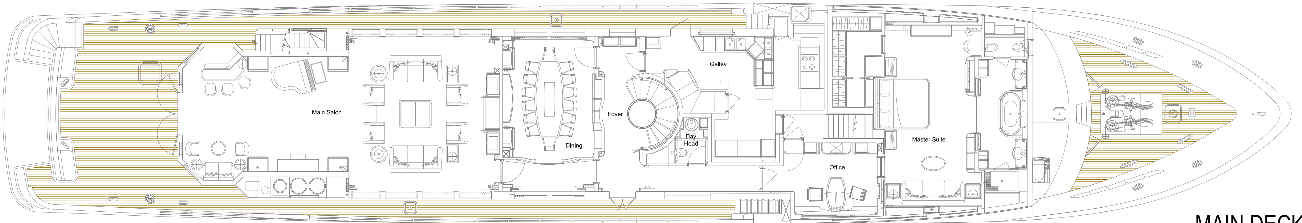
MAIN DECK
